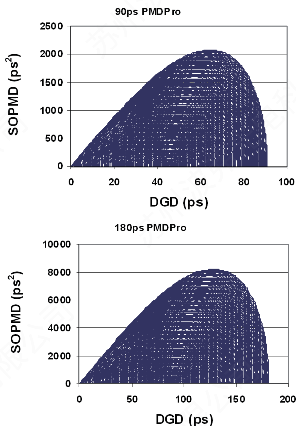
Figure 7 DGD and wavelength independent SOPMD range
