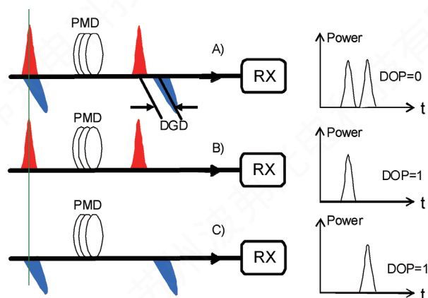
Figure 1 Illustrations of the PMD effect on an optical signal. A) The SOP of the input signal is aligned 45 degrees from the PSP of the fiber link, causing the worst-case signal distortion. In this case, if the DGD is larger than the width of one bit, then the DOP=0 because the two orthogonal polarization components have the same power, with no phase relationship. B) and C) The SOP of the input signal is aligned with the slow or fast PSP axis, respectively. In these cases, no signal distortion occurs except the slight late or early arrival, respectively, of the pulse. The DOP of the signal remains at 1. In all 3 cases, the PMD of the link remains the same, but the effect on the signal is different due to the different input polarization states.
