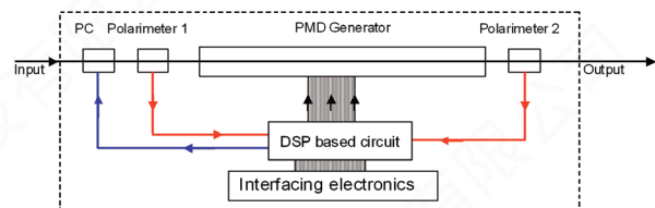
Figure 5 System diagram of polarization optimized PMD source. The DSP based circuit is used to 1) process information from the polarimeters and control instructions from users, 2) instruct the PMD generator to select desired PMD values, 3) control the PC to optimize the input SOP for various functions.
