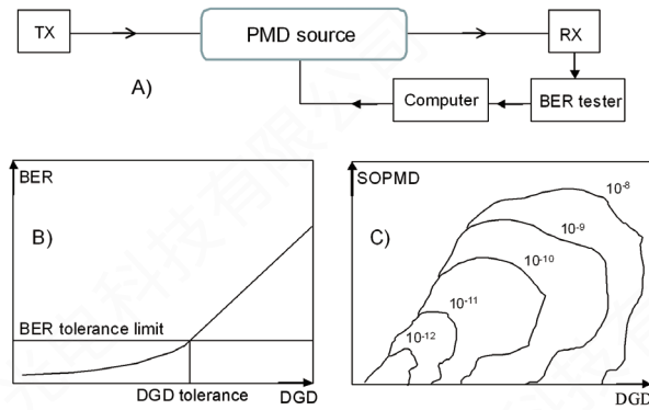
Figure 3 A) PMD tolerance test setup using a PMD source. The computer selects PMD settings and collects BER readings. B) BER vs. DGD curve. The DGD tolerance of the system for a given BER threshold can be deduced using the curve. C) Map of BER vs. DGD and SOPMD. Each contour represents a BER value. The PMD tolerance can be obtained from the contour plot.
