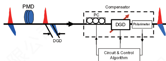
Figure 2 Optical PMD compensation. The DOP measured by the polarimeter is used as PMD effect indicator.
