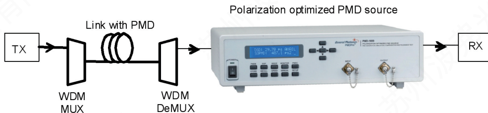
Figure 8 Polarization optimized PMD source in an in-service WDM link for the determination of its PMD and diagnosis of performance issues.
